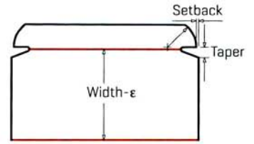
Slot Lock Tuck
