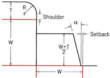
Friction Lock Tuck Dust Flaps
